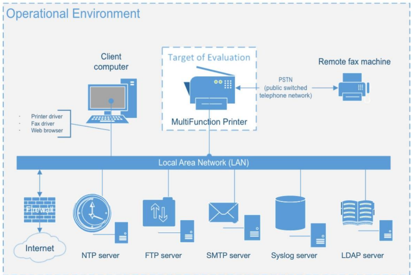
Figure 1: TOE Architecture
